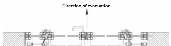
Door system during fire (evacuation) -sliding door opened permanently -fire-resistant door closed automatically, but may be opened manually with an anti-panic lever
