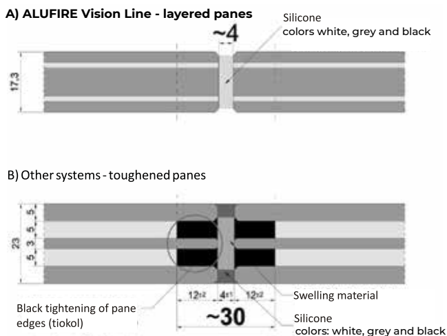
Figure 1. Total width of non-transparent strips on connections of layered pane of Alufire Vision Line (A) and toughened panes of other systems (B) - comparison.
