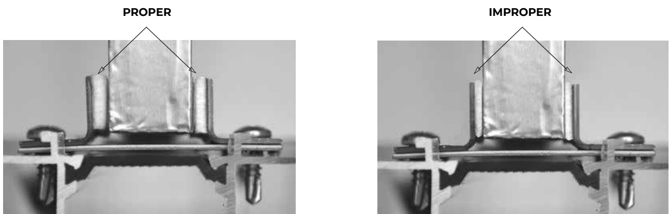
Photo 14. Proper mounting (felt washer, not deformed) and improper mounting (lack of clearance caused by non-parallel screwing of steel angle bar or by use of inappropriate angle bar)
